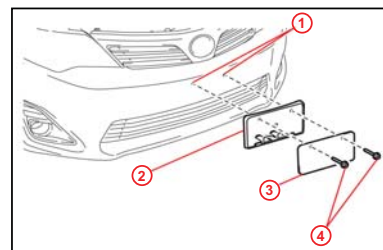
1 Dimples 2 Front License Plate Mounting Bracket 3 License Plate 4 Self-tapping Screws
