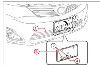
1 Air Intake 2 Hooks 3 Front License Plate Mounting Bracket 4 Tab 5 Rotate Bracket
